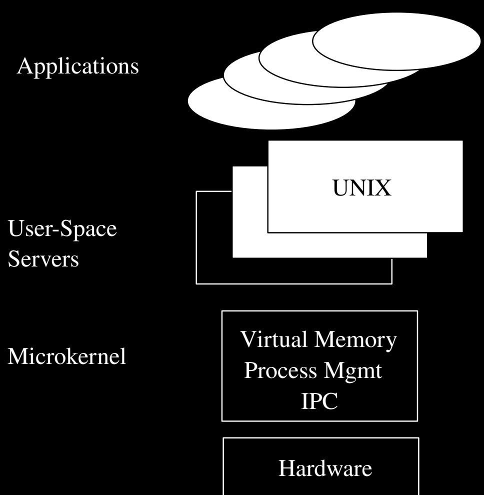
Microkernel
